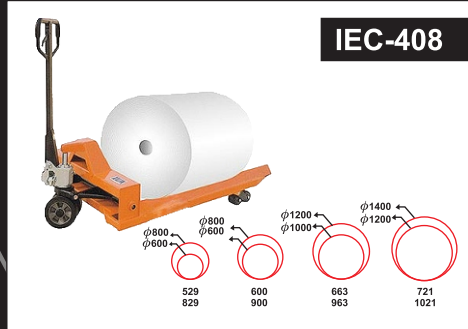
Reel Pallet Truck As Per Customer Requirement
